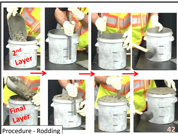
Procedure - Rodding
