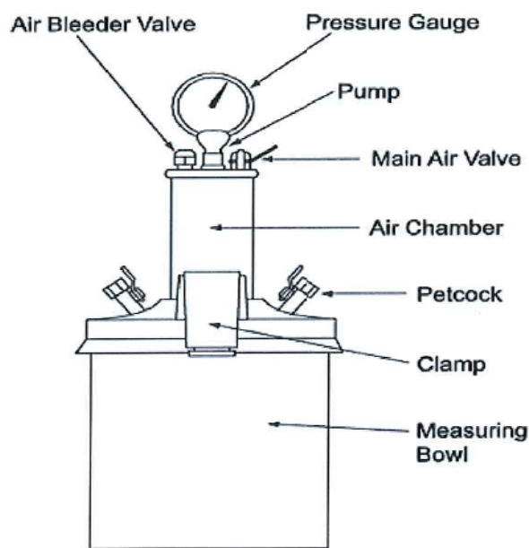
2b. Vertical Air Chamber
