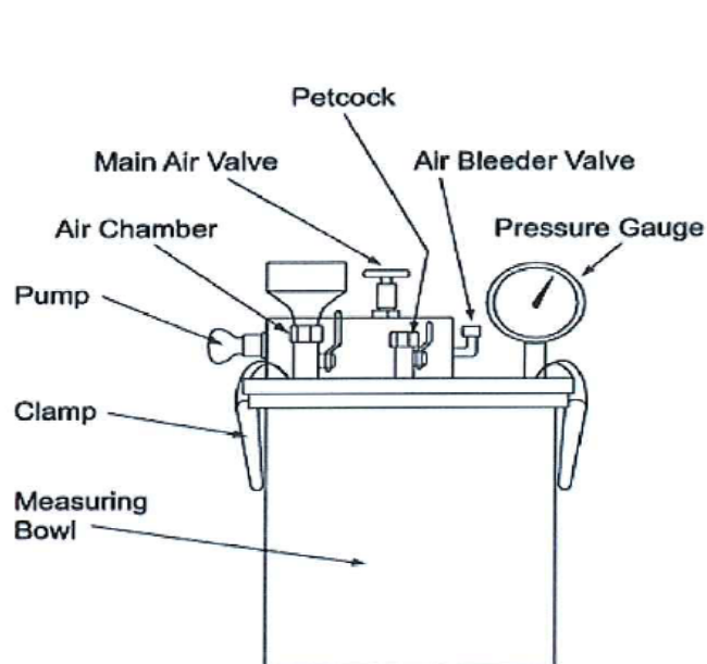
2a. Horizontal Air Chamber
