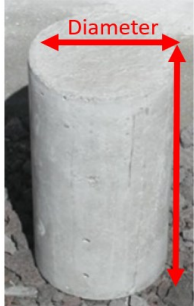
Fig.1: Concrete Cylinder for Compression Test
